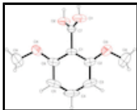
Fig. 1. The molecular structure of (I), showing the atom-labelling scheme. Displacements ellipsoids are at the 50% probability level.
