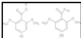
Fig. 3. A scheme showing antiplanar and synplanar conformations of the carboxy group.
